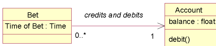
Figure 52 - Datatypes added
