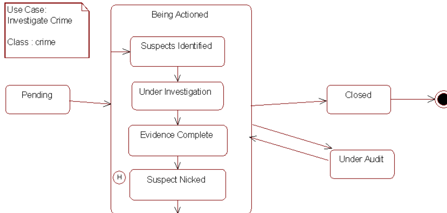
Figure 102 - History State
