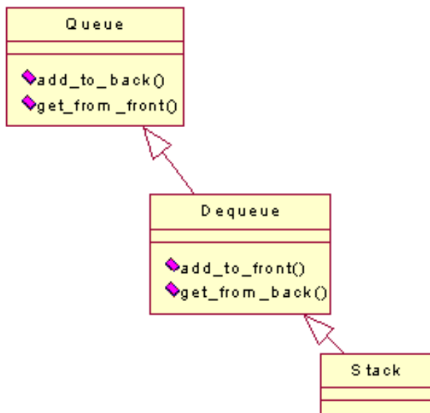
Figure 77 - Creating a Stack...no work needed!
