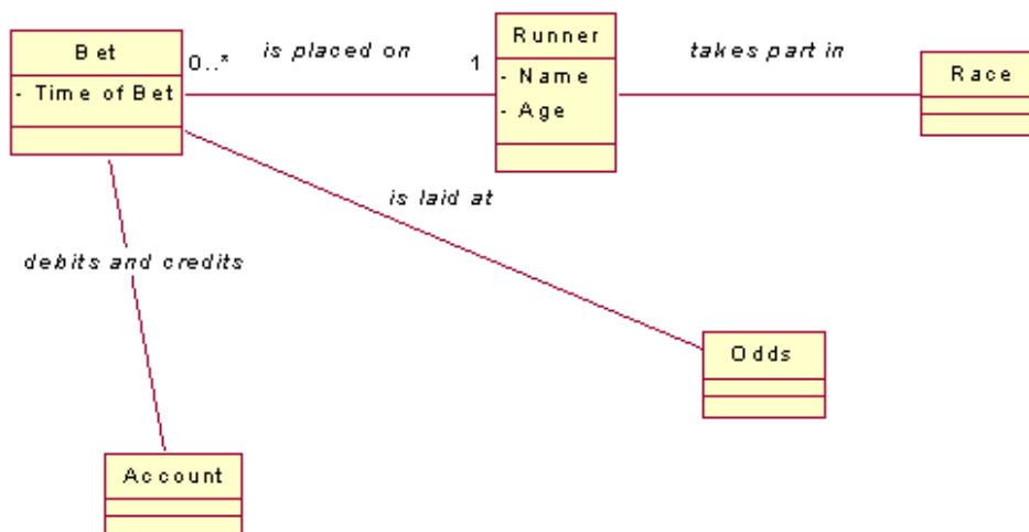
Figure 47 - Betting System Conceptual Model
