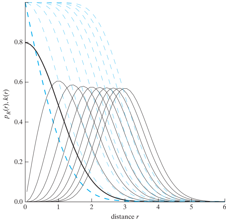
FIGURE 9.14 Two different sets of plots versus the distance r are shown in the figure for unit variance and increasing dimensionality m = 1, 2, 3, \dots :
