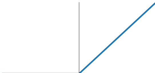
Figure 3.3 ReLU
