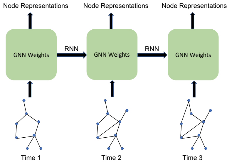
Figure 8.3 An illustration for EvolveGCN
