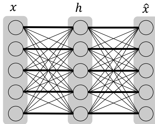
Figure 3.15 An autoencoder memorizes the input to the output. The bold connection indicates the memorization from the input to the output and the other connections are not used (with weights 0) in the autoencoder.
