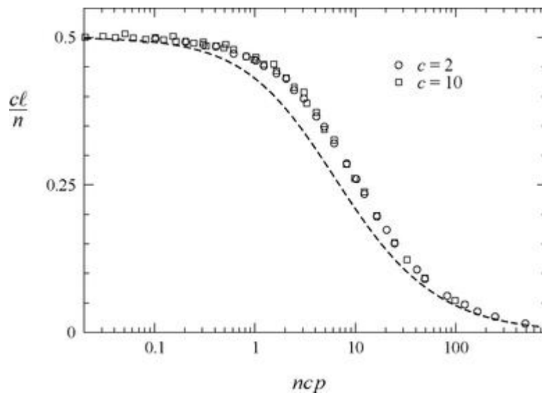
Figure 15.6: Scaling function for the small-world model. The points show numerical results for c\ell/n as a function of n c p for the small-world model with a range of parameter values n = 128 to 32\,768 and p = 1 \times 10^{-6} to 3 \times 10^{-2} , and two different values of c as marked. Each point is averaged over 1000 networks with the same parameter values. The points collapse, to a reasonable approximation, onto a single scaling function f(ncp) in agreement with Eq. (15.13). The dashed curve is the mean-field approximation to the scaling function given in Eq. (15.14).
