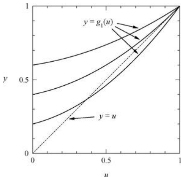
Figure 13.6: Graphical solution of Eq. (13.91). The solution of the equation u = g_1(u) is given by the point at which the curve y = g_1(u) intercepts the line y = u .
