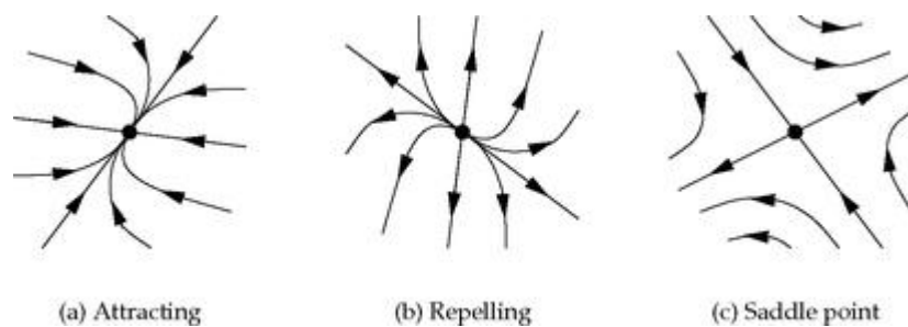
Figure 18.2: Examples of flows around general fixed points. When the Jacobian matrix is not diagonal the flows around a fixed point look like squashed or stretched versions of those in Fig. 18.1.
