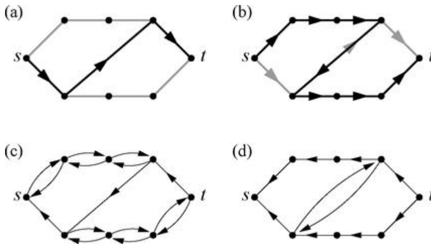
Figure 10.6: The augmenting path algorithm. (a) We find a first path from source s to target t using breadth-first search. This leaves no more independent paths from s to t among the remaining edges. (b) However, if we allow flows in both directions along an edge (such as the central edge in this network), then we can find another path. Panels (c) and (d) show the residual graphs corresponding to panels (a) and (b).
